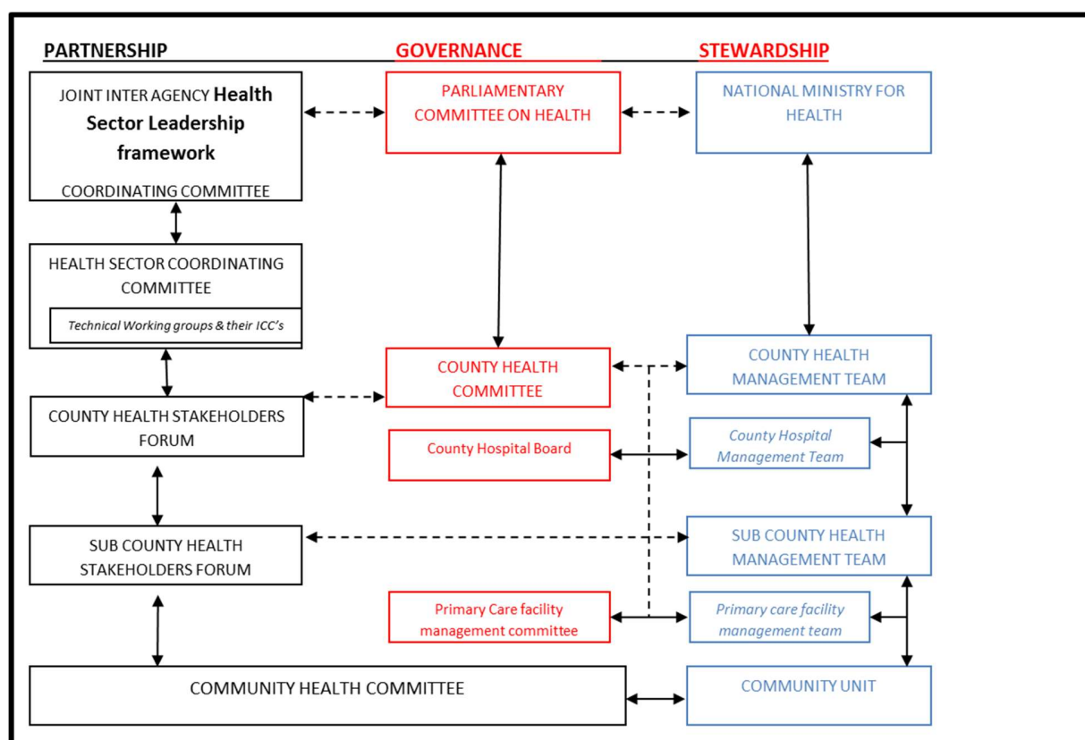
Figure 2: Coordination mechanism
